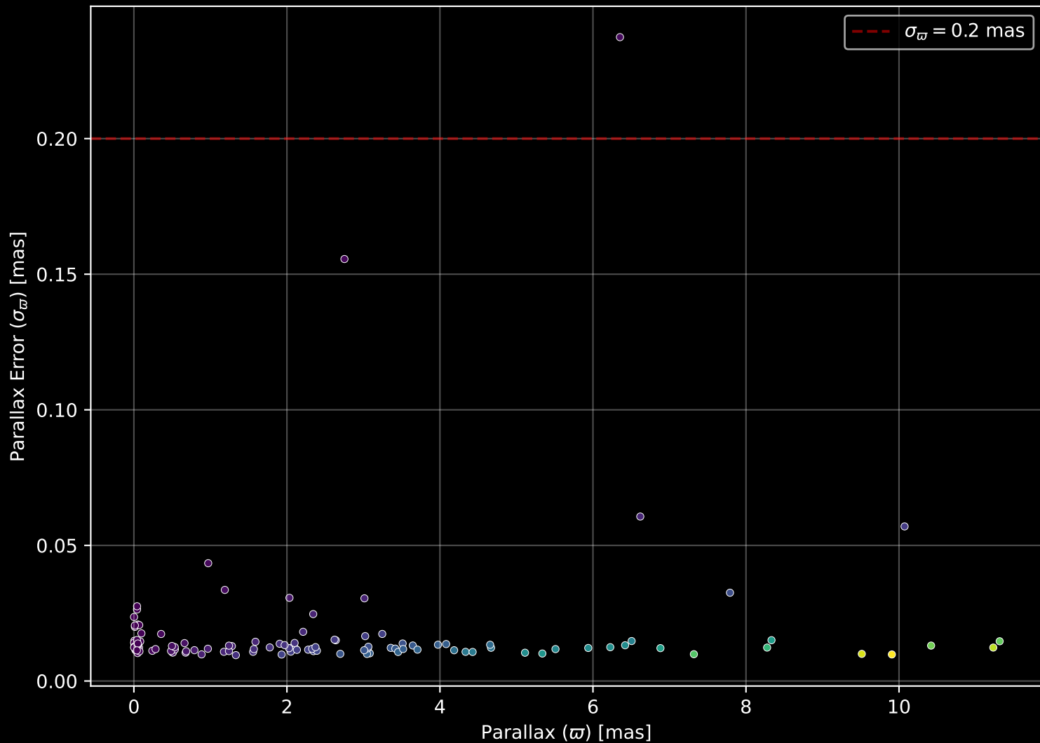
APOGEE DR17 Field: [279-32-O_TESS] Parallax Quality (n= 122)
