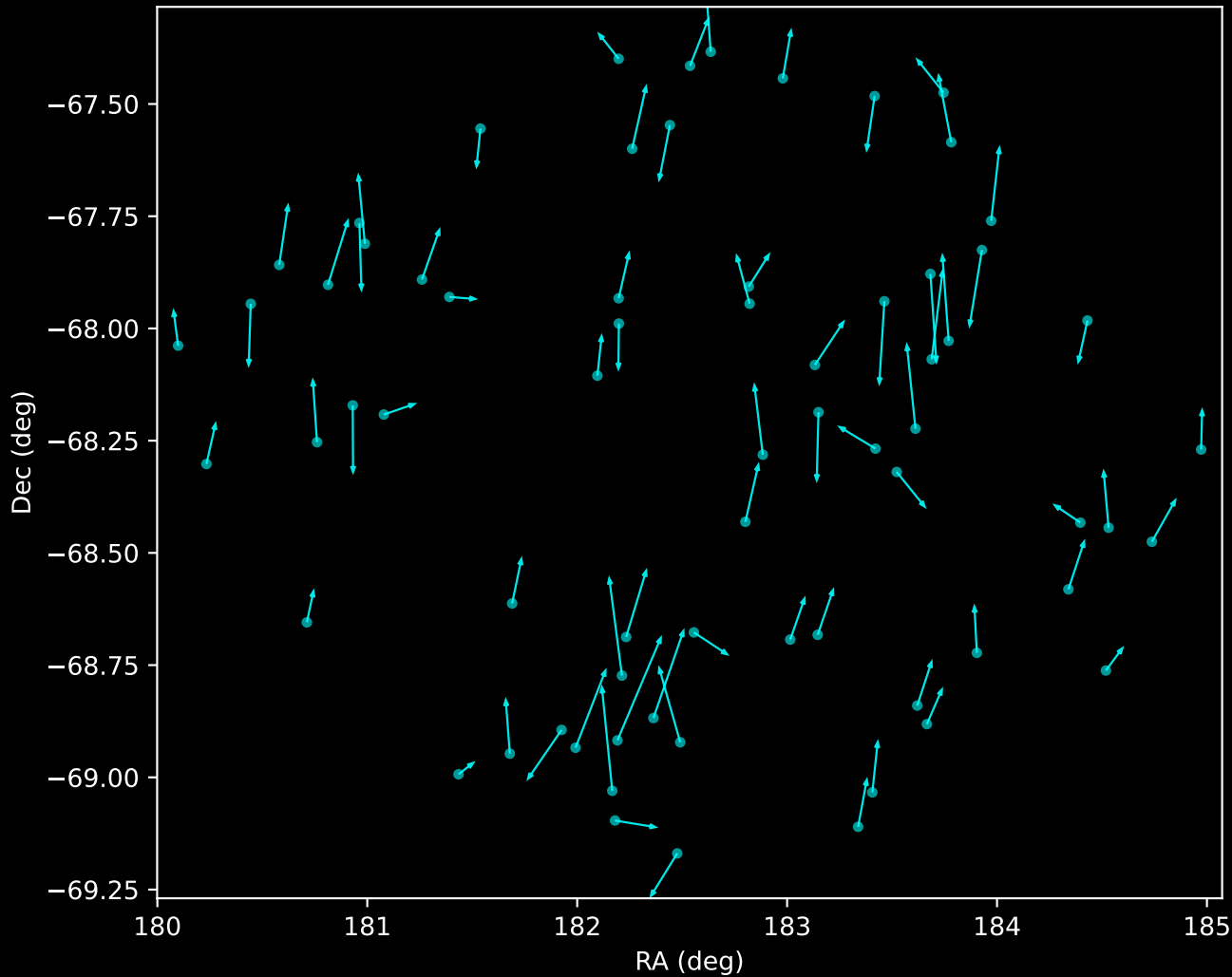
APOGEE DR17 Noise Stream Proper Motion Vectors (n=69)
