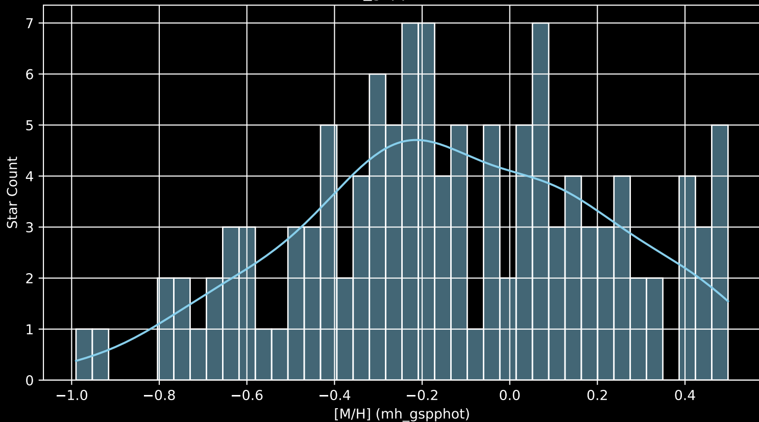
APOGEE DR17 Field: [279-32-O_TESS [M/H] (mh_gspphot) (n= 121)
