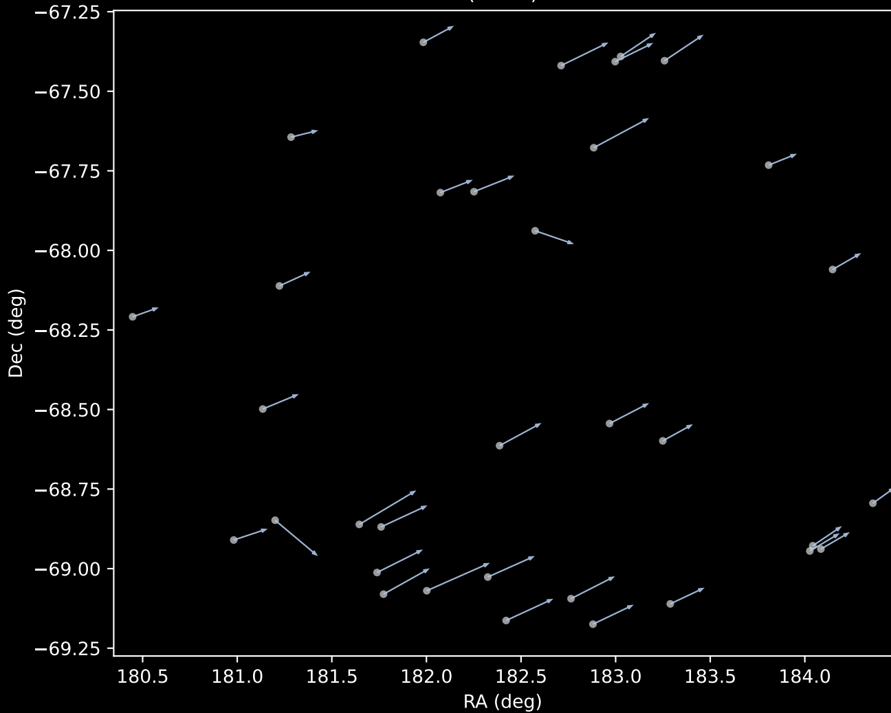
APOGEE DR17 Cluster 1 Proper Motion Vectors (n=34)
