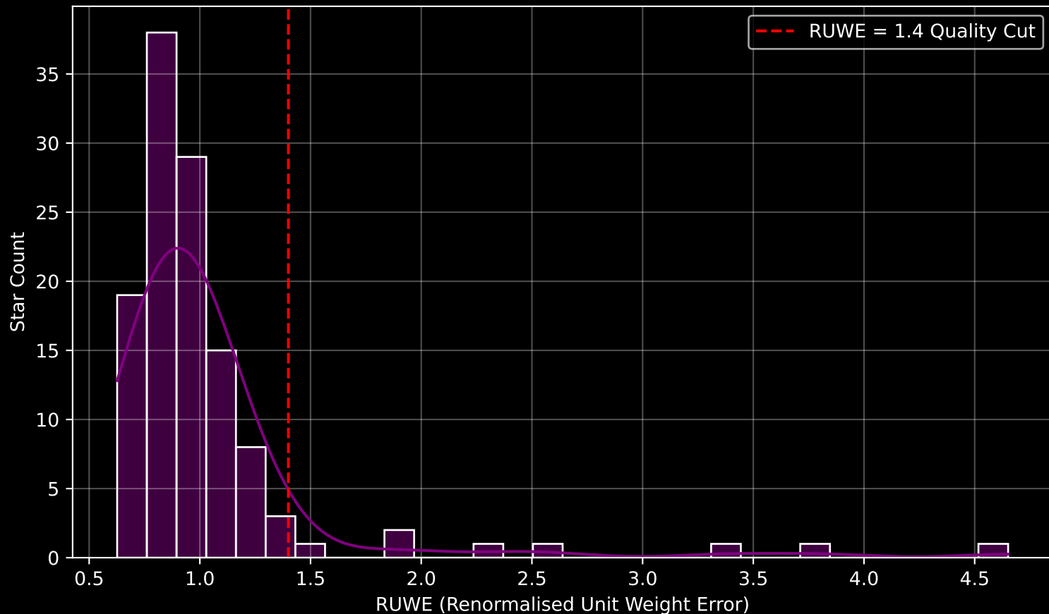
GAPOGEE DR17 Field [279-32-O_TESS] RUWE Distribution (n= 120)
