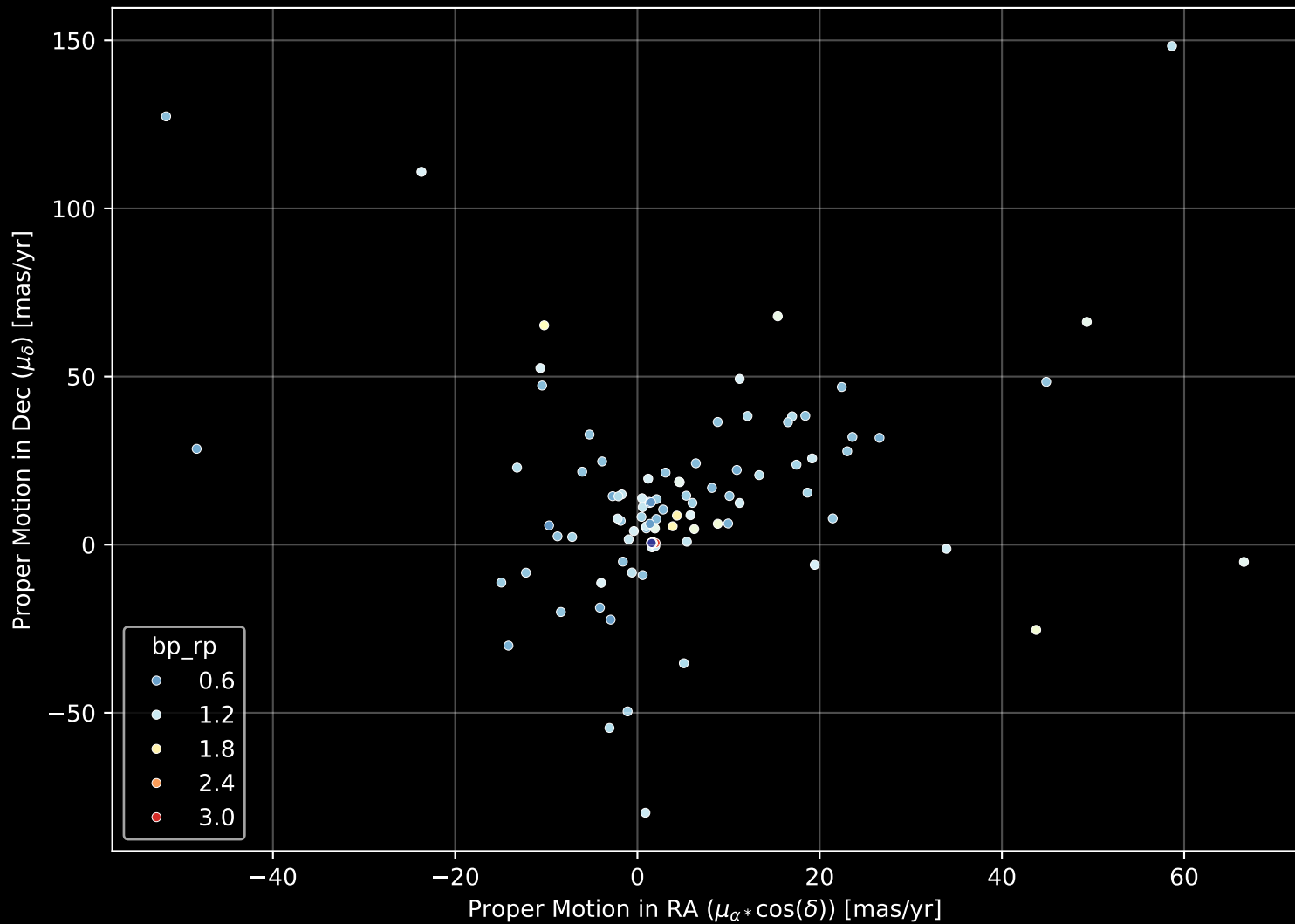
APOGEE DR17 Field: [279-32-O_TESS] Proper Motion Diagram (n= 122)
